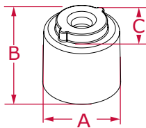
QSP1 Quick-Lock Spacer A: 18.5mm B: 15.5mm C: 12mm
